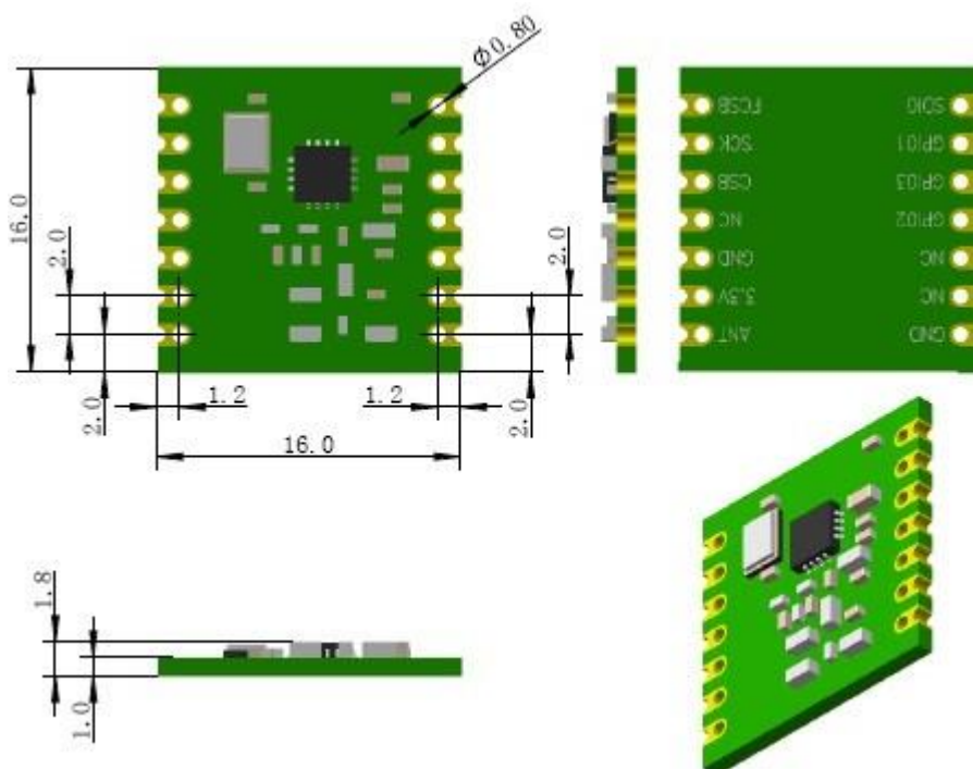
Figure3. CYF300W Mechanical Dimension
