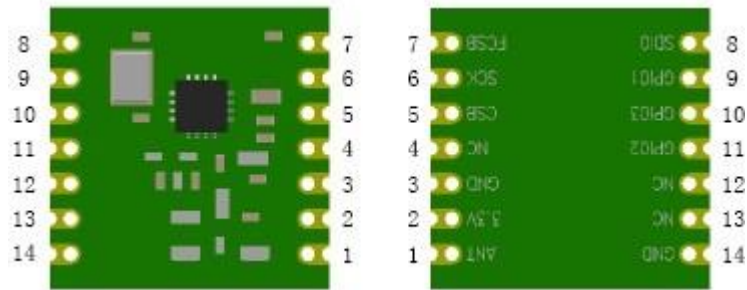
Figure 1. CYF300W Pin Definition
